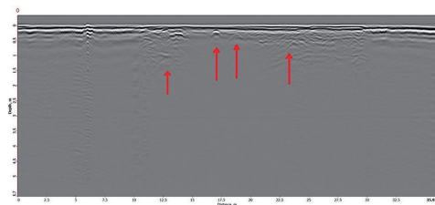
Example of a GPR profile produced using RadSys Zond 12e, with marked parabolas, most likely indicating underground utility lines (author: A. Zelenkevičs)
