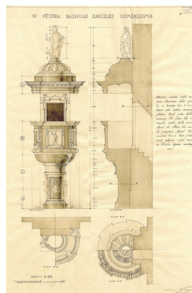
St. Peter's Church pulpit measurement. NHB collection
