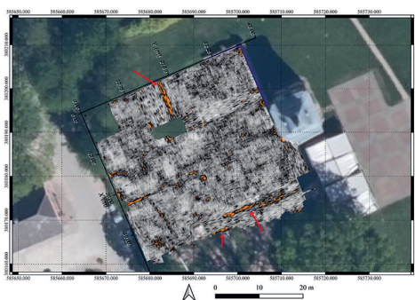
Depth map with marked old structures or pieces of foundations produced using IDS GeoRadar RIS MF Hi-Mod (author: A. Zelenkevičs)
